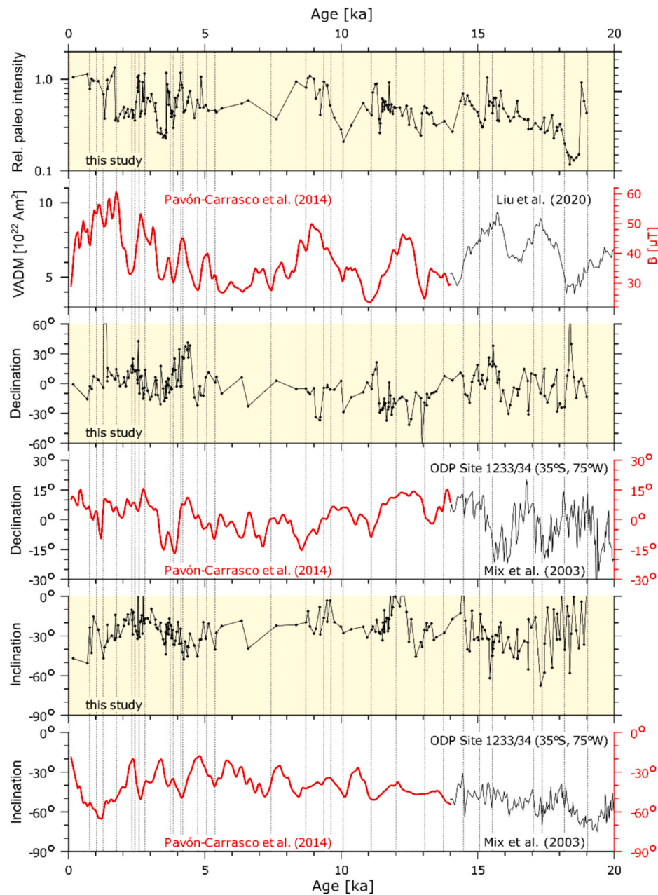
Fig. 5. Magnetostratigraphic results (light yellow background) including relative paleointensity (slope (NRM/ARM)), declination (ChRM), and inclination (ChRM), along with the comparison with marine records (Mix et al., 2003; Liu et al., 2020) and geomagnetic field models (Pavón-Carrasco et al., 2014). VADM = Virtual axial dipole moment. Tie points are indicated by vertical dashed lines. (For interpretation of the references to colour in this figure legend, the reader is referred to the web version of this article.)
