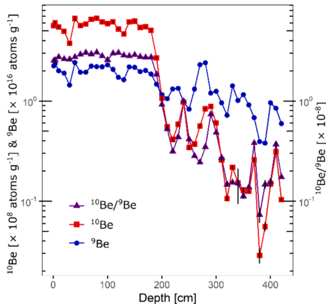
Fig. 7. Beryllium isotope concentrations and ratios (not corrected for radioactive decay) along the profile depth. Average ^{10}\text{Be} fluxes are 3 orders of magnitudes lower than in the CP interval, with \Phi(^{10}\text{Be}_{\text{dc}}) = 9.3 \times 10^3 atoms cm ^{-2} a ^{-1} , while the average calcium sulfate flux is one order of magnitude lower, with \Phi(\text{CaSO}_4) = 0.31 g m ^{-2} a ^{-1} (Table 3).
