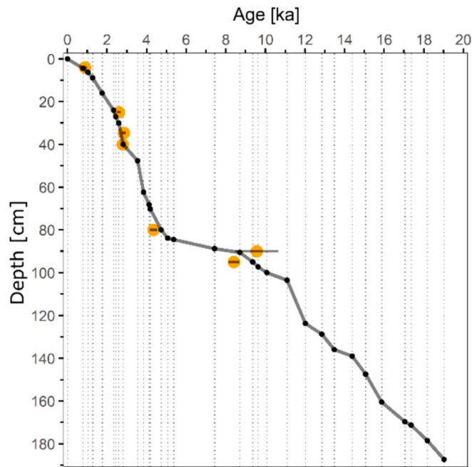
Fig. 6. CP depositional dating results. A) Depositional ages from radiocarbon dating of H. fruticose seeds (yellow dots with gray uncertainty bars) and magnetostratigraphy (gray line) with tie points (black dots and dashed vertical line) (Fig. 5). (For interpretation of the references to colour in this figure legend, the reader is referred to the web version of this article.)
