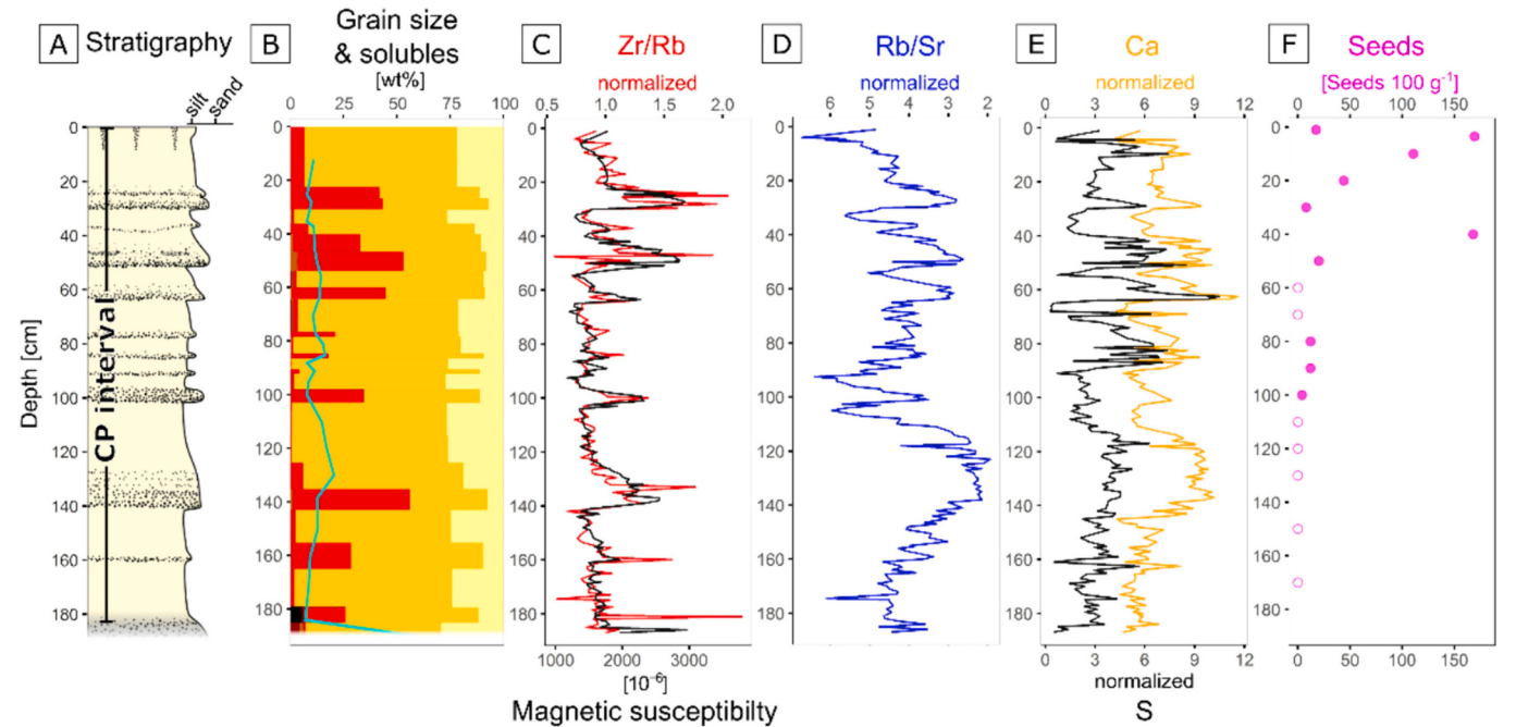
Fig. 3. Additional results covering the CP interval. A) Stratigraphy, for legend see Fig. 2. B) Grain size distribution and soluble content for the CP interval, for legend see Fig. 2. C) Zr/Rb ratio (red line) and magnetic susceptibility ( \kappa_{LF} ) given in SI units ( 10^{-6} ) (black line) (see Fig. 4). D) Rb/Sr ratio. E) Ca and S concentrations. F) Huidobria fruticosa seed abundance (purple dots), purple circles indicate that no seeds were found. (For interpretation of the references to colour in this figure legend, the reader is referred to the web version of this article.)
