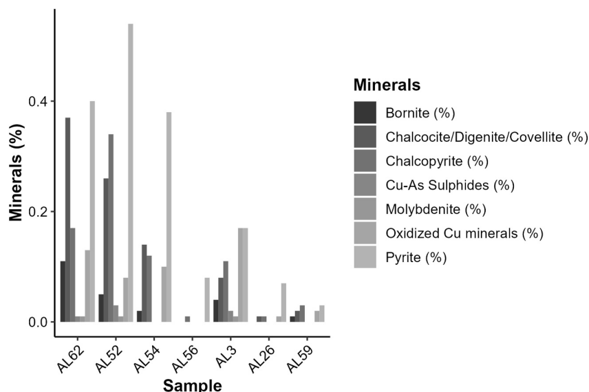
Figure 6. Mineralogy (sulfide phases) of the <75 \mu\text{m} fraction (wtf) of selected surface sediment samples as a function of the distance from the possible pollution sources (Distance < 20 km: Samples AL62, AL52, and AL54; Distance 20–40 km: Samples AL56 and AL3; Distance >40 km: Samples AL26 and AL59). See Figure 1 for the location of the samples used for this analysis.
